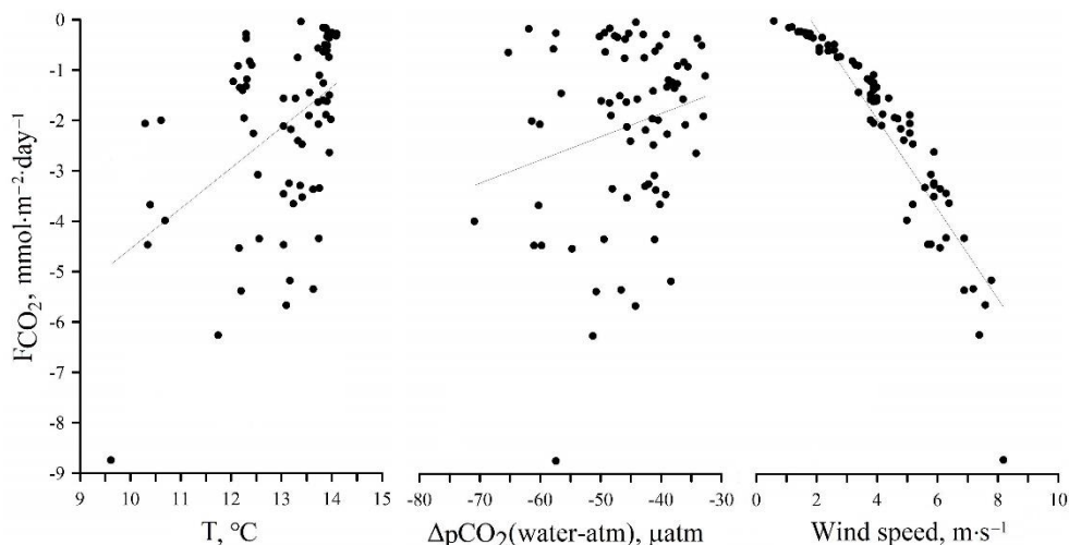
Fig. 3. Dependence of \text{CO}_2 flux ( F_{\text{CO}_2} ) on temperature, \Delta p\text{CO}_2 and wind speed
