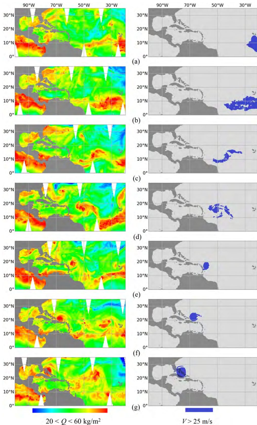
Figure 8: Evolutions of the total atmospheric water vapor content Q and near-surface wind speed V fields: (a) – 22.08; (b) – 24.08; (c) – 26.08; (d) – 28.08; (e) – 30.08; (f) – 01.09; (g) – 03.09. White wedge-shaped areas are the blind spots of the AMSR-E radiometer resulted from the divergence of its scanning bands. A tropical wave is detected by the AMSR-E radiometer 5 days before the hurricane Frances origin (26.08.2014).
