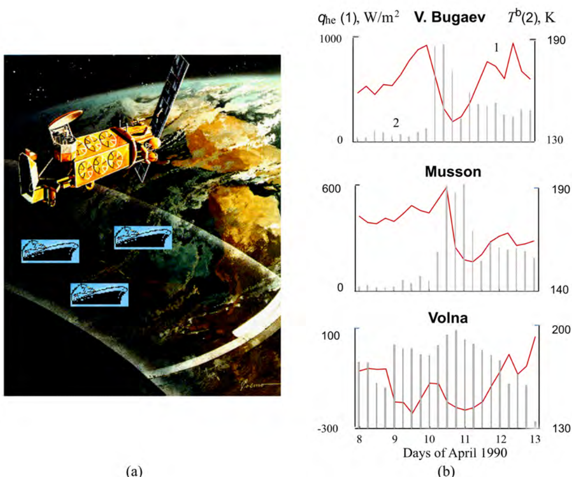
Figure 1: MCW radiometric survey of the meteorological satellite F08 in areas of carrying out of experiments NEWFOUEX-88 and ATLANTEX-90 aboard the research vessels V. Bugaev, Musson and Volna in the Newfoundland energy active zone of the North Atlantic (a). Variations of the surface total heat fluxes q_{he} (1) (in Watts per square meter) according to ship measurements carried out on the vessels V. Bugaev (42.3°N, 46°W), Musson (41.3°N, 41°W) and Volna (48.2°N, 46°W) in the experiment ATLANTEX-90 and brightness temperature T^b at the wavelength 1.35 cm (2) from the F08 SSM/I radiometer (b). There are clear relations between brightness temperature and heat fluxes variations.
