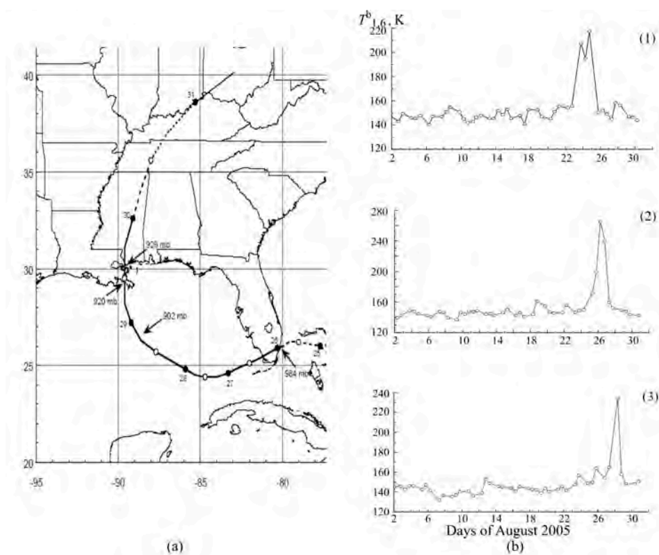
Figure 4: Trajectory of hurricane Katrina propagation from the area of its arising; figures are the days of August 2005 [Knabb et al., 2023] (a). Variations of the brightness temperature T^b at the wavelength 1.6 cm on the horizontal polarisation measured by AMSR-E radiometer at several points of Katrina trajectory: 1) (26°N, 78°W); 2) (25°N, 83°W); 3) (27°N, 89°W) (b). The movement of the brightness temperature peaks in the Bermuda area and in the Gulf of Mexico coincides with the trajectory of the hurricane.
