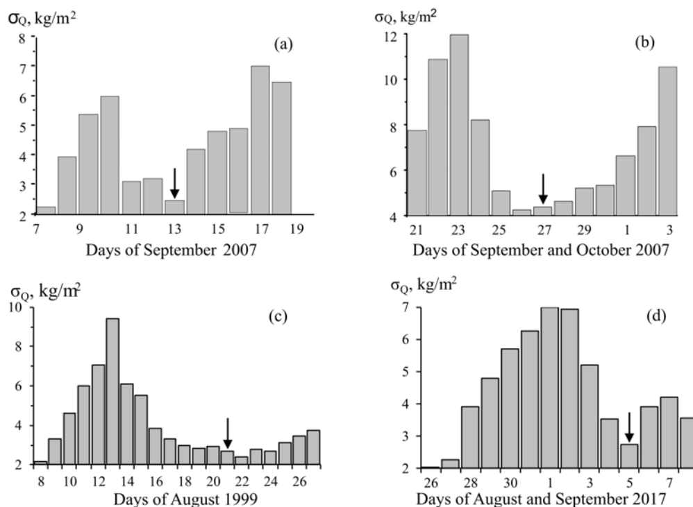
Figure 7: Standard deviations of the total atmospheric moisture content \sigma_Q from the daily average values in the Gulf of Mexico during the periods of origin and development of the Humberto (a), Lorenzo (b), Bret (c) and Katia (d) hurricanes. The arrow marks the moment of transition of the tropical formations to the hurricane stage. A smoothing of atmospheric water vapor fields in the Gulf before the hurricanes origin is observed.
