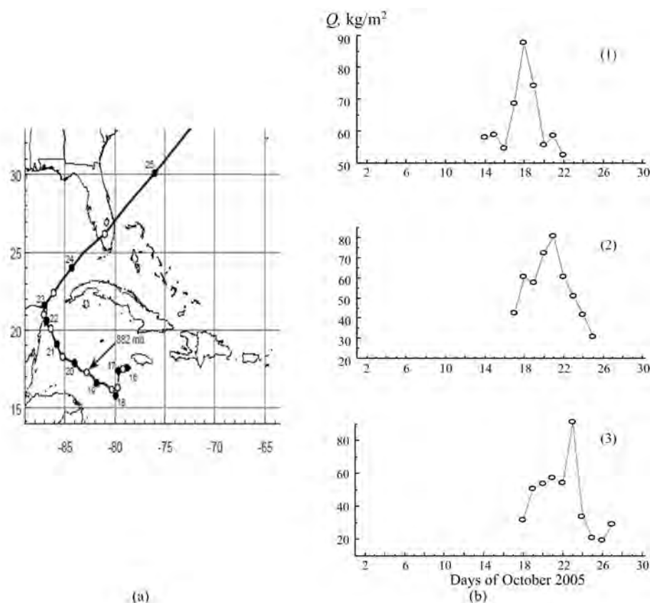
Figure 5: Trajectory of hurricane Wilma propagation from the area of its arising: figures are the days of October 2005 [Pasch et al., 2006] (a). Variations of the atmosphere total water vapor content Q derived from AMSR-E radiometer at several points of Wilma trajectory: 1) (15.8°N, 79.9°W); 2) (19.1°N, 85.8°); 3) (24°N, 84.3°) (b). The movement of the atmospheric water vapor peaks in the in the Caribbean Sea and in the Gulf of Mexico coincides with the trajectory of the hurricane.
