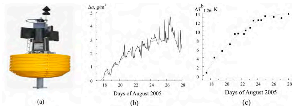
Figure 2: NOAA network buoy station SMKF1 (a). Variations of the near-surface air humidity \Delta a (in grams per cubic meter) according to the station SMKF1 measurements (24.38°N, 81.07°W) (b) and SOA brightness temperature \Delta T^b at the wavelength of 1.26 cm (c) with the data from the EOS Aqua AMSR-E radiometer in August 2005.
