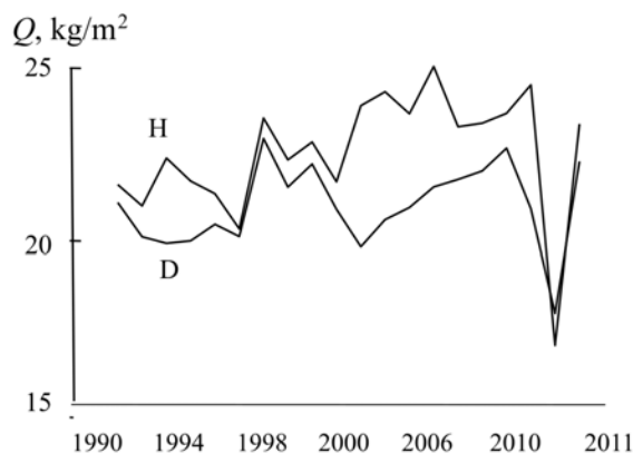
Figure 10: Dynamics of changes in the total water vapor content in the atmosphere Q and its peculiarity in 2010. There is a sharp decrease in the average annual values of the total water vapor content in the atmosphere in the D and H regions of the North Atlantic after the beginning of oil spills in May 2010.
