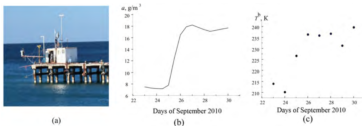
Figure 3: Pier with installed complex of meteorological sensors in the Blue Bay of the Black sea (Gelendzhik), September 2010. Increase in the near-surface air humidity a (according to meteorological measurements made in September 2010 from the pier in the Blue Bay of the Black sea) (a) and the SOA brightness temperature T^b at the wavelength 1.26 cm (data obtained by the EOS Aqua AMSR-E radiometer) (b).
