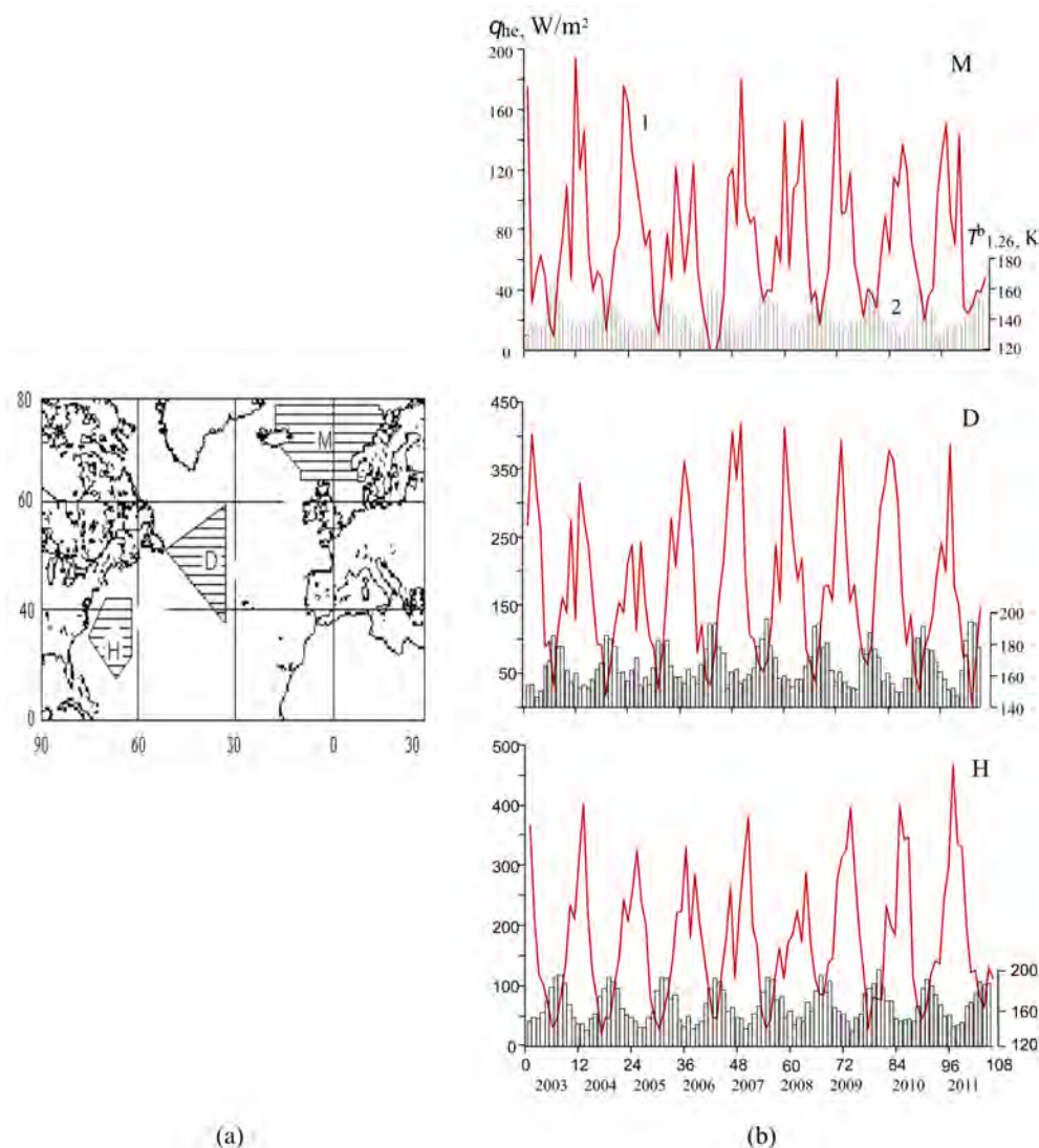
Figure 9: Location of Norwegian, Newfoundland, and Gulf Stream active zones and the ocean weather stations M, D, and H in the North Atlantic (a). Comparison of the OAFlux monthly mean fluxes of total heat q_{he} and AMSR-E brightness temperatures T^b at the wavelength 1.26 cm in the areas M, D, H during 2003–2011 (b). A high correlation between seasonal and interannual variations in average monthly heat fluxes on the sea surface and brightness temperatures are observed in the areas M, D, H of the North Atlantic.
