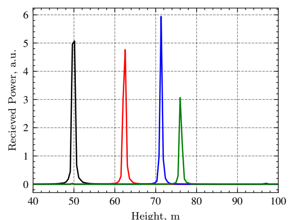
Figure 8: Changing the position of the pulse when moving over the Volga River.
