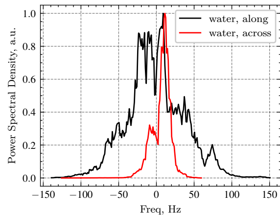
Figure 12: Doppler spectra of the reflected radar signal over the water surface for orienting the knife-like antenna across the direction of movement (red curve) and along the direction of travel (black curve).
