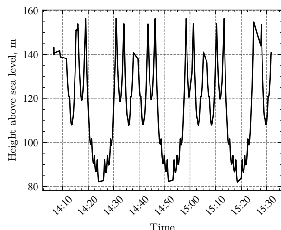
Figure 4: Changing the height of the technological trolley (radar) during the experiment.
