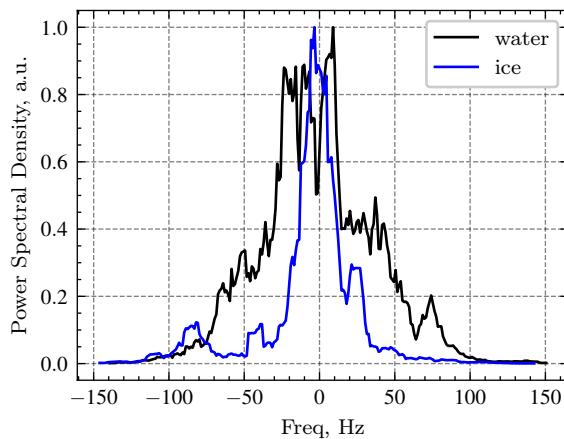
Figure 11: An example of Doppler spectra reflected from the water surface (black curve) and from the ice cover (blue curve).
