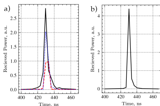
Figure 6: An example of a reflected pulse: a) single reflected pulses; b) average pulse. The height of the technological trolley is about 64.5 m.
