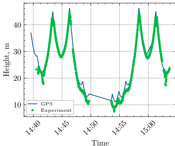
Figure 9: Dependence of the height of the technological trolley on time: GNSS is solid line, radar data is dots.
