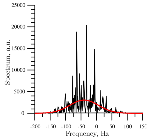
Figure 7: Doppler spectrum of the reflected signal: black curve – measured Doppler spectrum, red curve – Gaussian model. Time record is 0.7 s.
