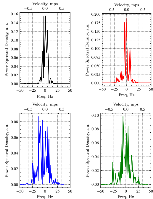
Figure 10: Examples of Doppler spectra of the reflected radar signal.
